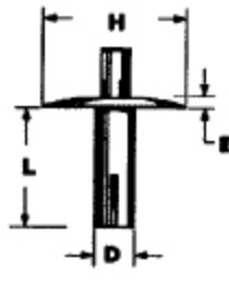
RIVET SIZE SPECIFICATIONS AND HOLE SIZE DATA
